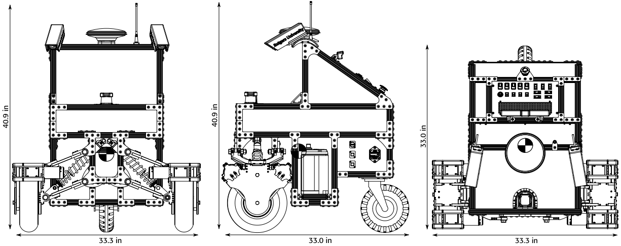
Figure 3: Mechanical drawing of Navi generated from the detailed CAD model. Note how the center of mass (denoted by a checkered circle) is located near the axis of rotation.
