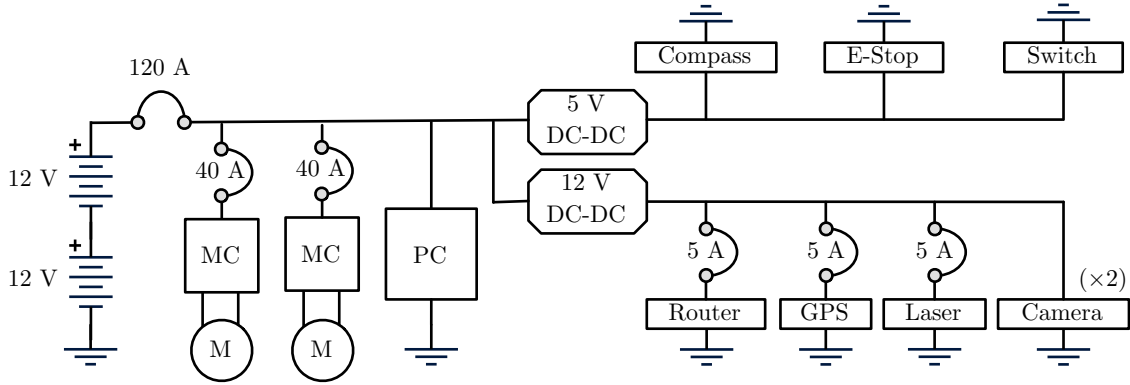
Figure 5: High level wiring diagram for Navi. Thermal circuit breakers are labeled with their current and some come components are omitted for clarity.
