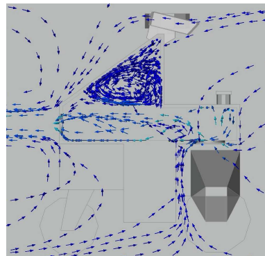
Figure 4: Airflow simulation.
